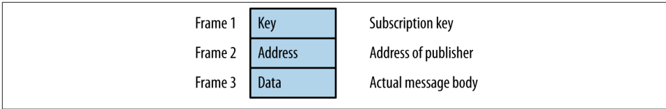
Figure 2-16. Pub-sub envelope with sender address
