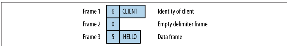
Figure 3-11. Message delivered to worker
