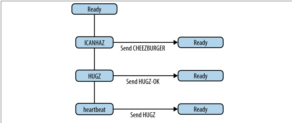
Figure 7-3. The “Ready” state
