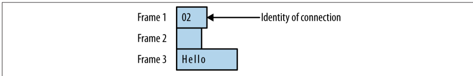
Figure 3-3. Request with one address
