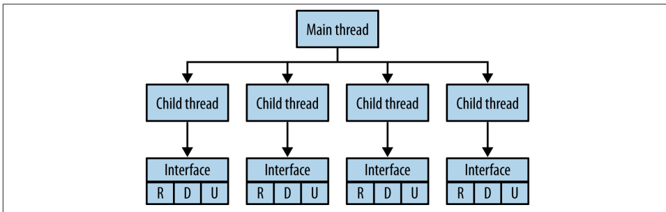
Figure 8-2. Zyre tester tool
